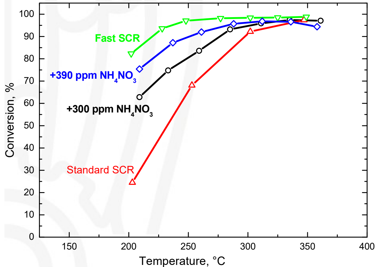
NOx Conversion vs temperature
